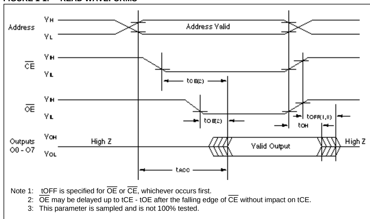
FIGURE 1-1: READ WAVEFORMS
