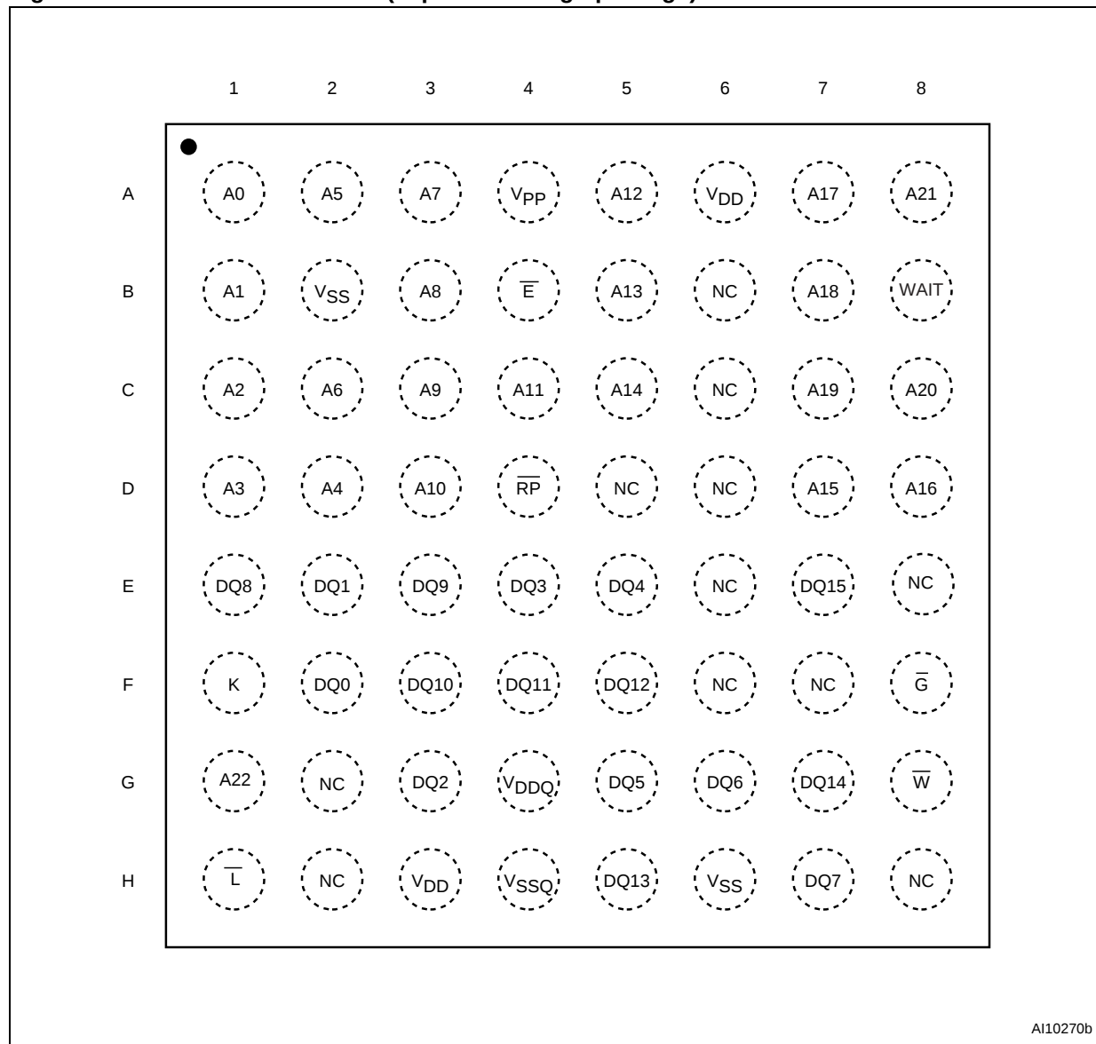
Figure 2. TBGA64 Connections (Top view through package)
