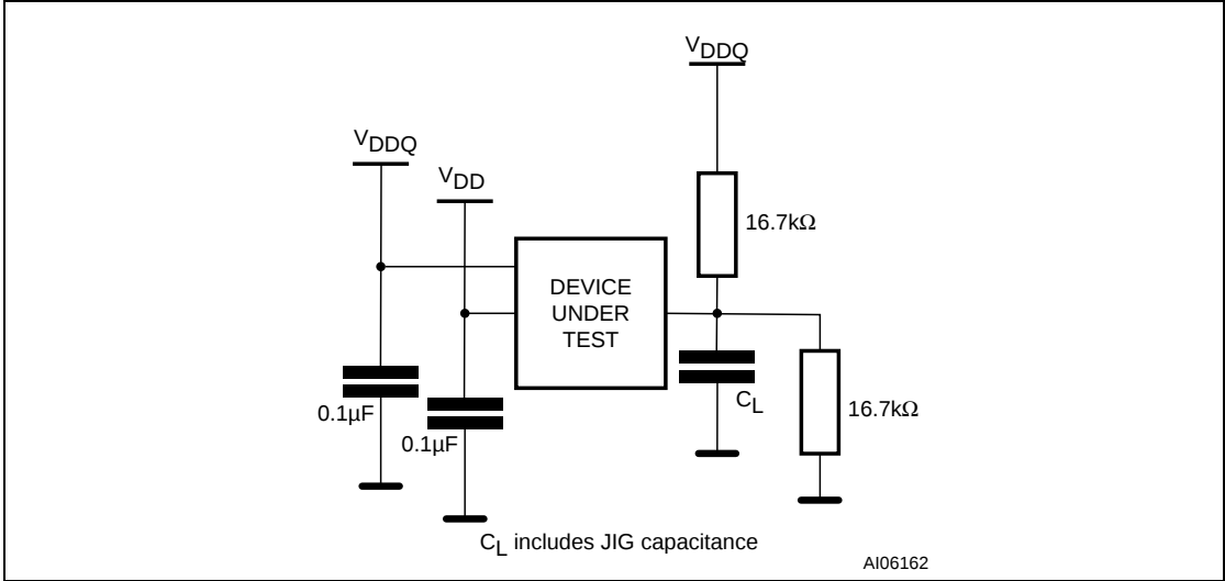
Figure 8. AC Measurement Load Circuit
