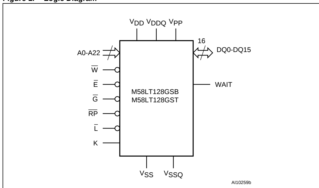
Figure 1. Logic Diagram
