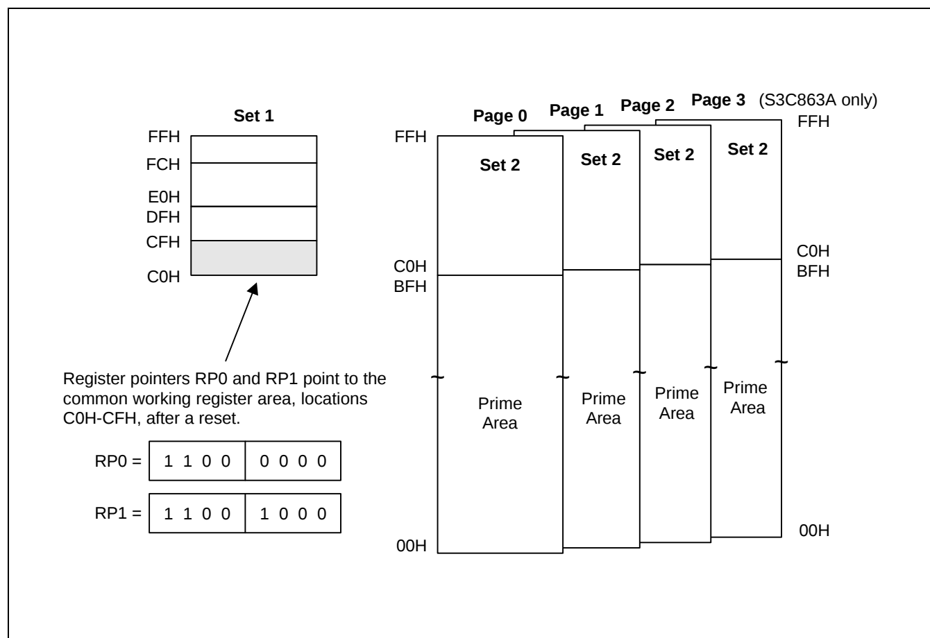
Figure 2-12. Common Working Register Area (S3C863X)
