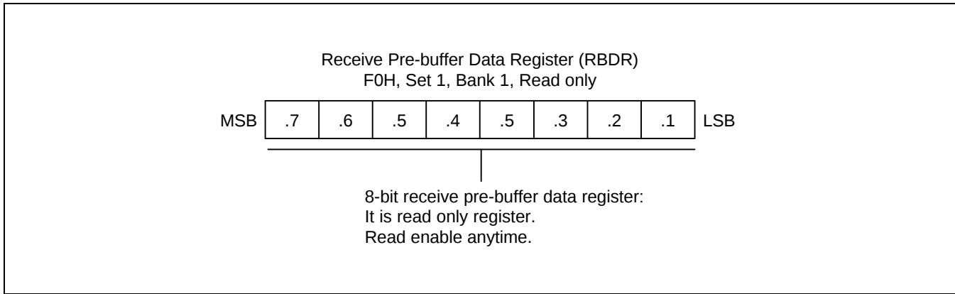
Figure 17-9. Receive Pre-buffer Data Register (RBDR)
