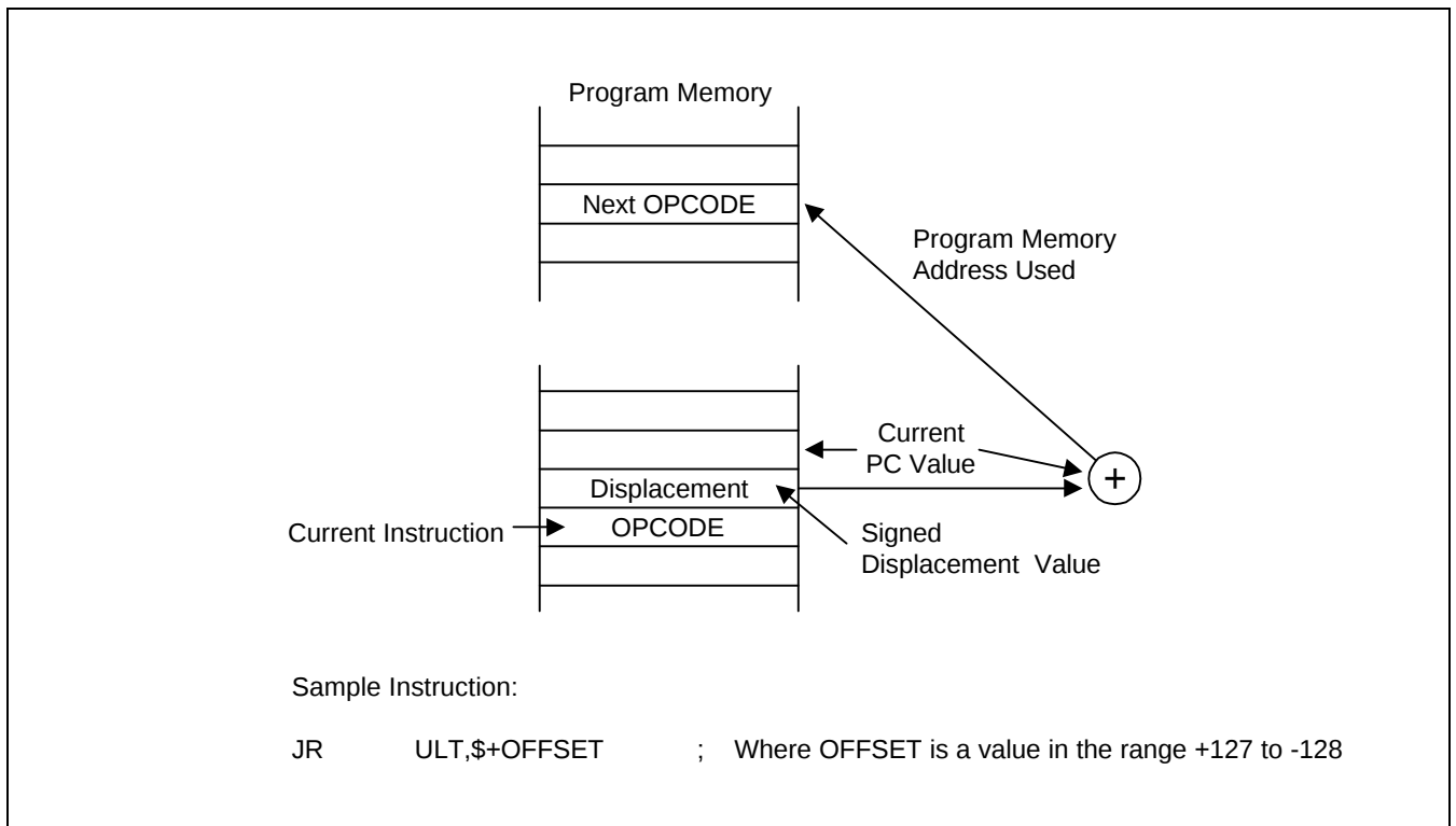
Figure 3-13. Relative Addressing
