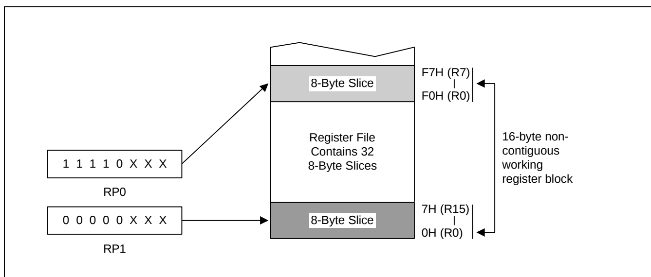
Figure 2-9. Non-Contiguous 16-Byte Working Register Block
