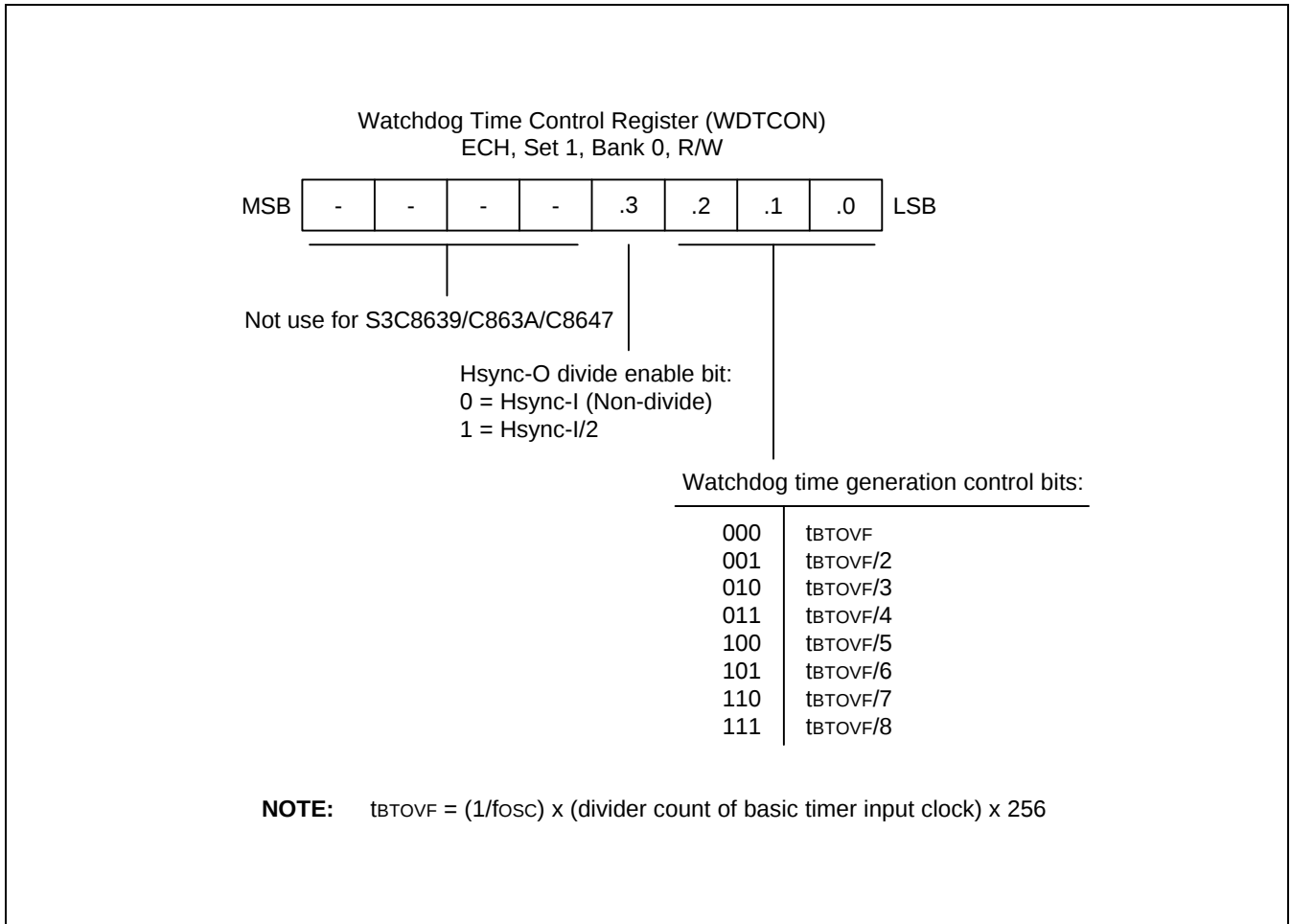
Figure 10-2. Watchdog Time Control Register (WDTCON)
