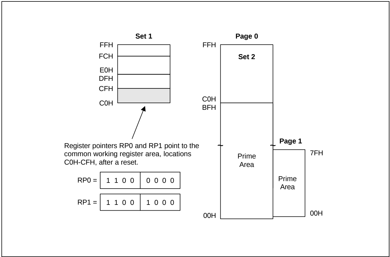
Figure 2-13. Common Working Register Area (S3C8647)
