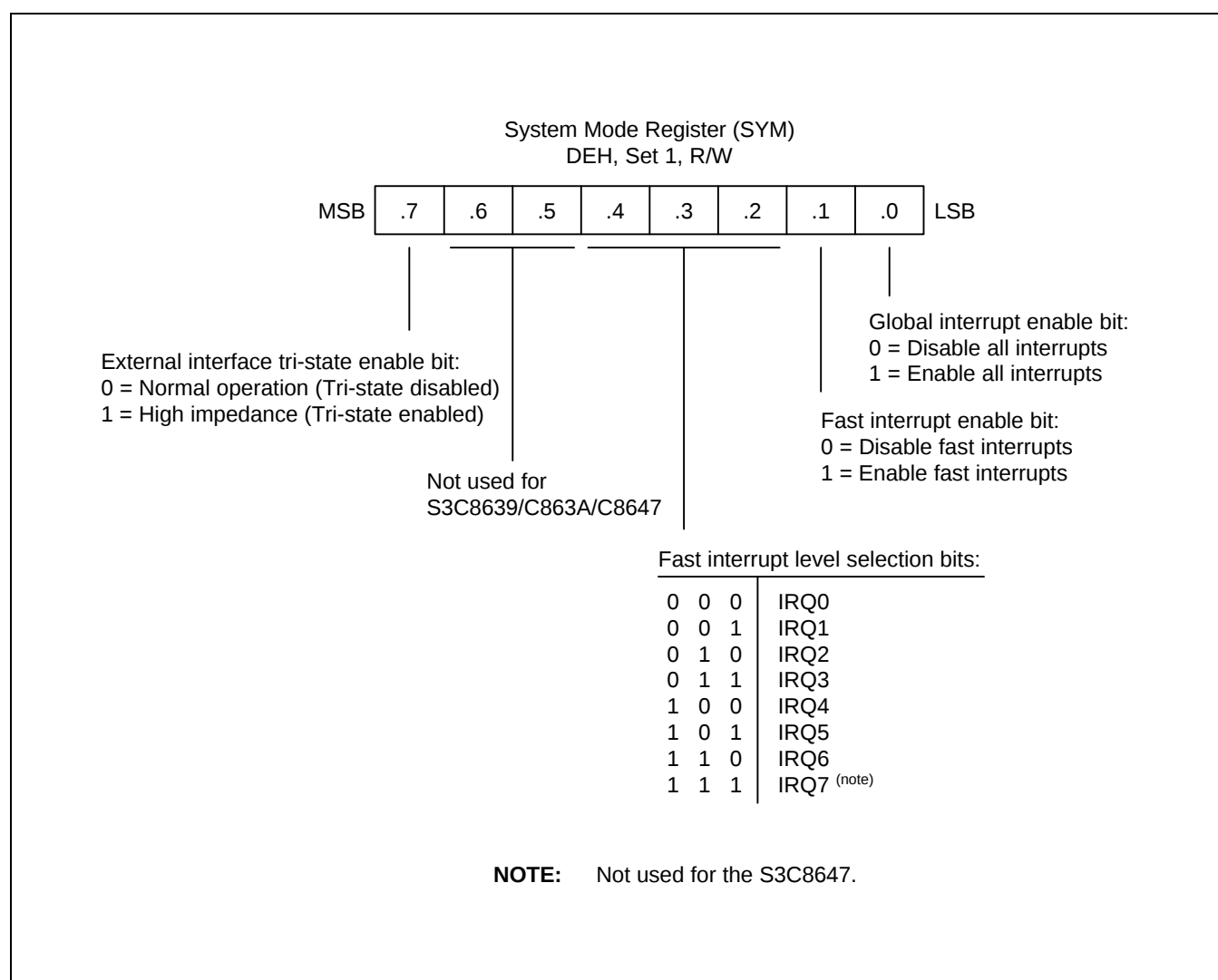
Figure 5-5. System Mode Register (SYM)
