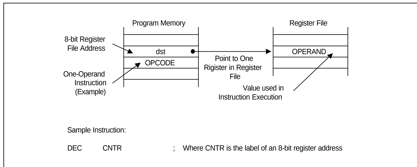
Figure 3-1. Register Addressing
