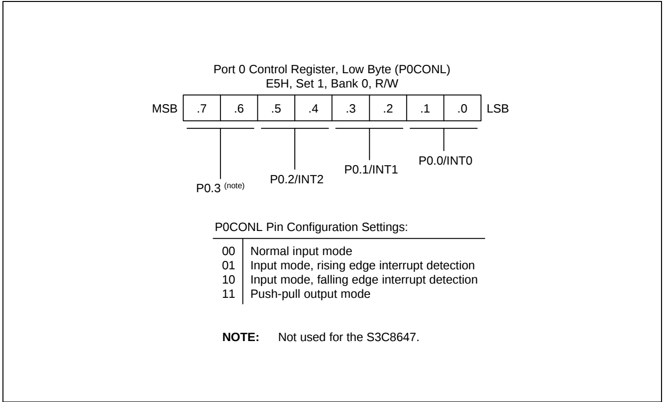
Figure 9-3. Port 0 Low-Byte Control Register (P0CONL)
