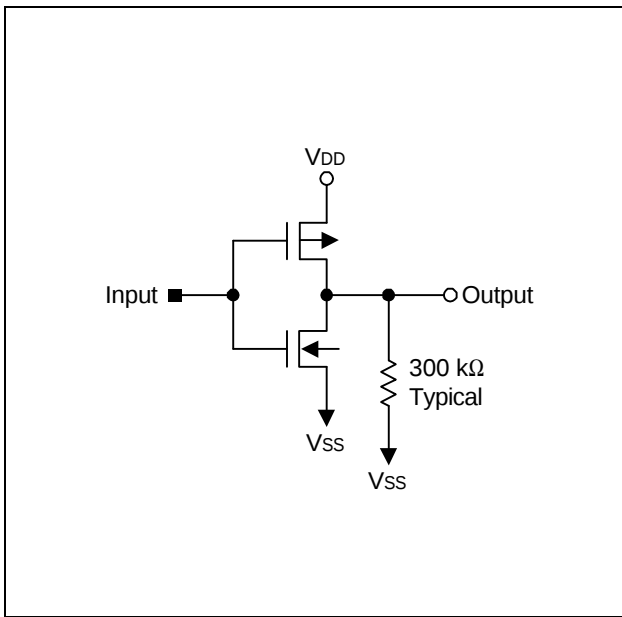
Figure 1-8. Pin Circuit Type A-3
