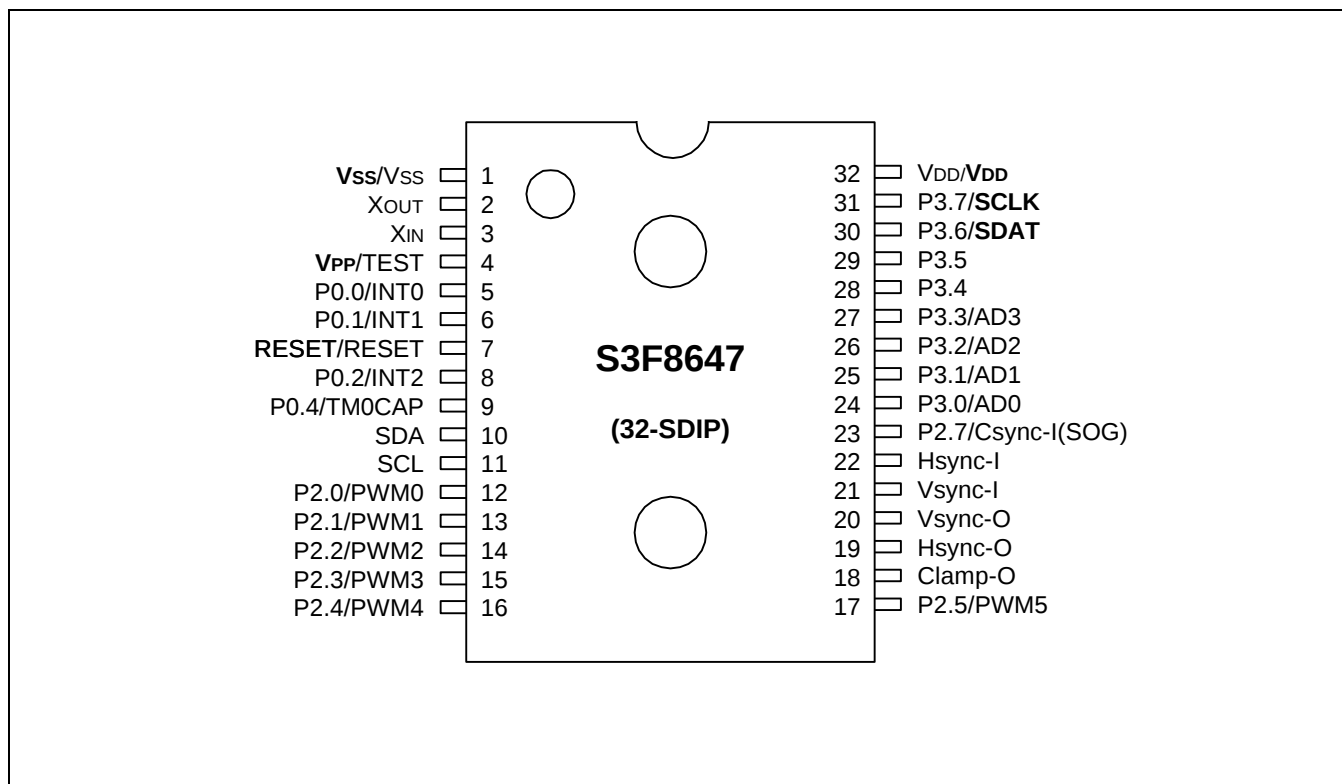
Figure 22-1. S3F8647 Pin Assignments (32-SDIP Package)
