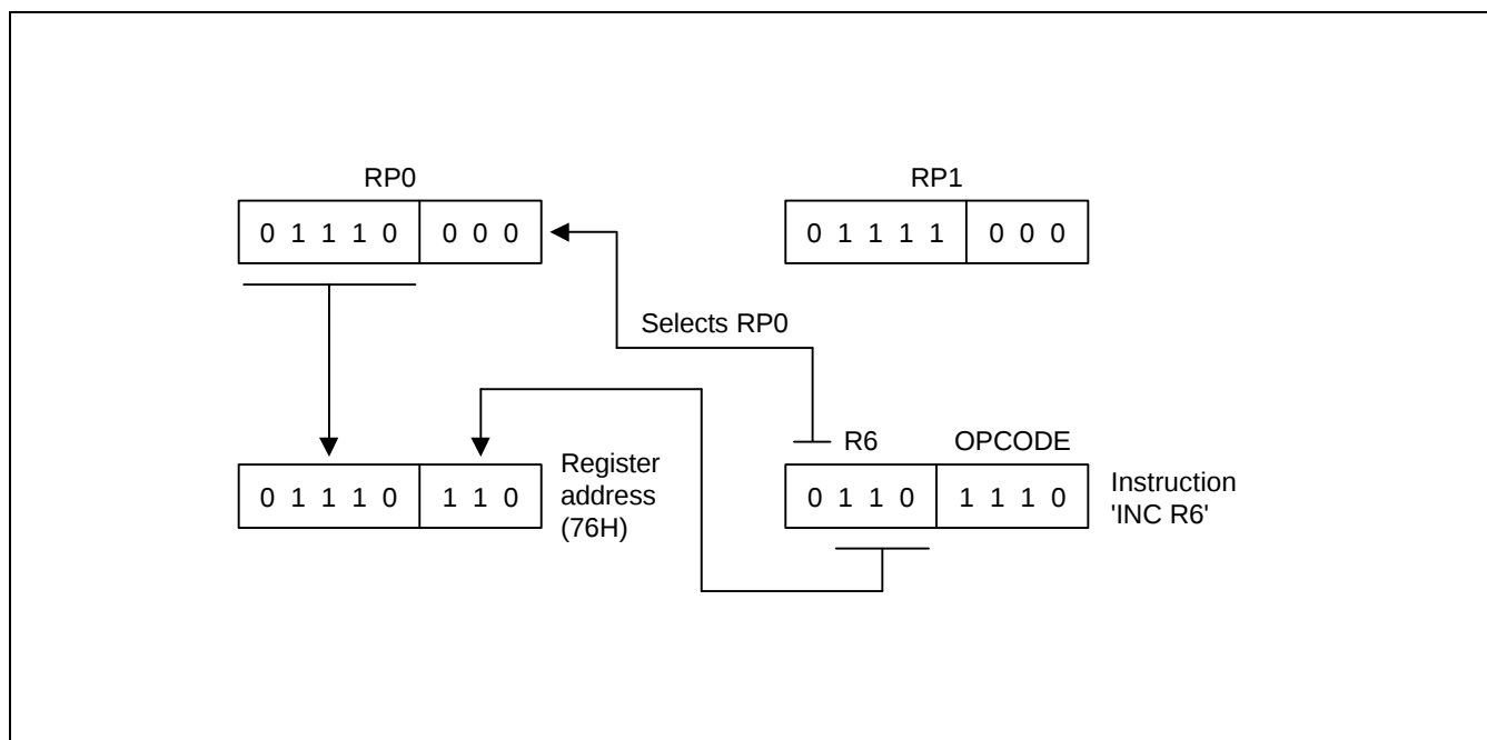
Figure 2-15. 4-Bit Working Register Addressing Example
