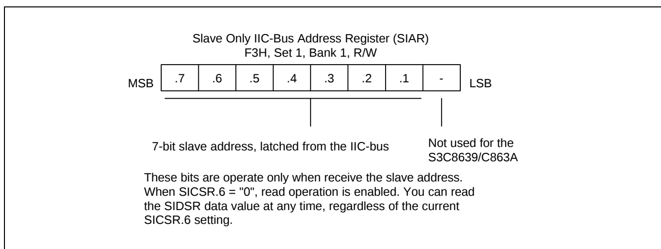
Figure 18-3. Slave only IIC-Bus Address Register (SIAR)
