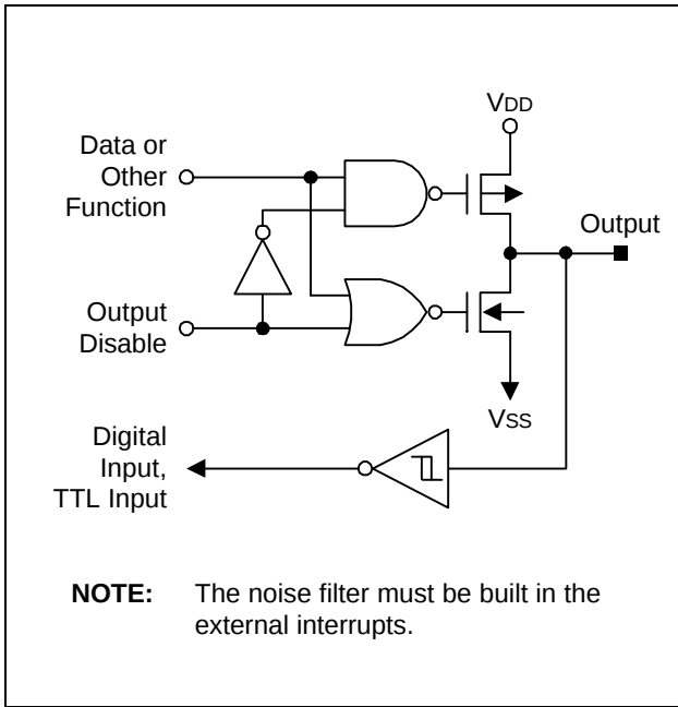
Figure 1-10. Pin Circuit Type D-1
