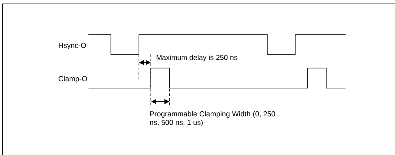
Figure 16-12. Clamp-O Signal Delay Timing
