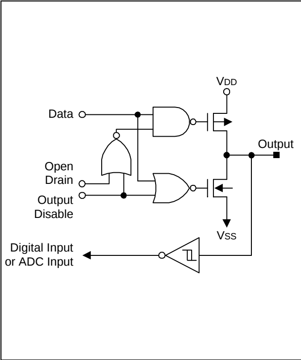
Figure 1-12. Pin Circuit Type E-1
