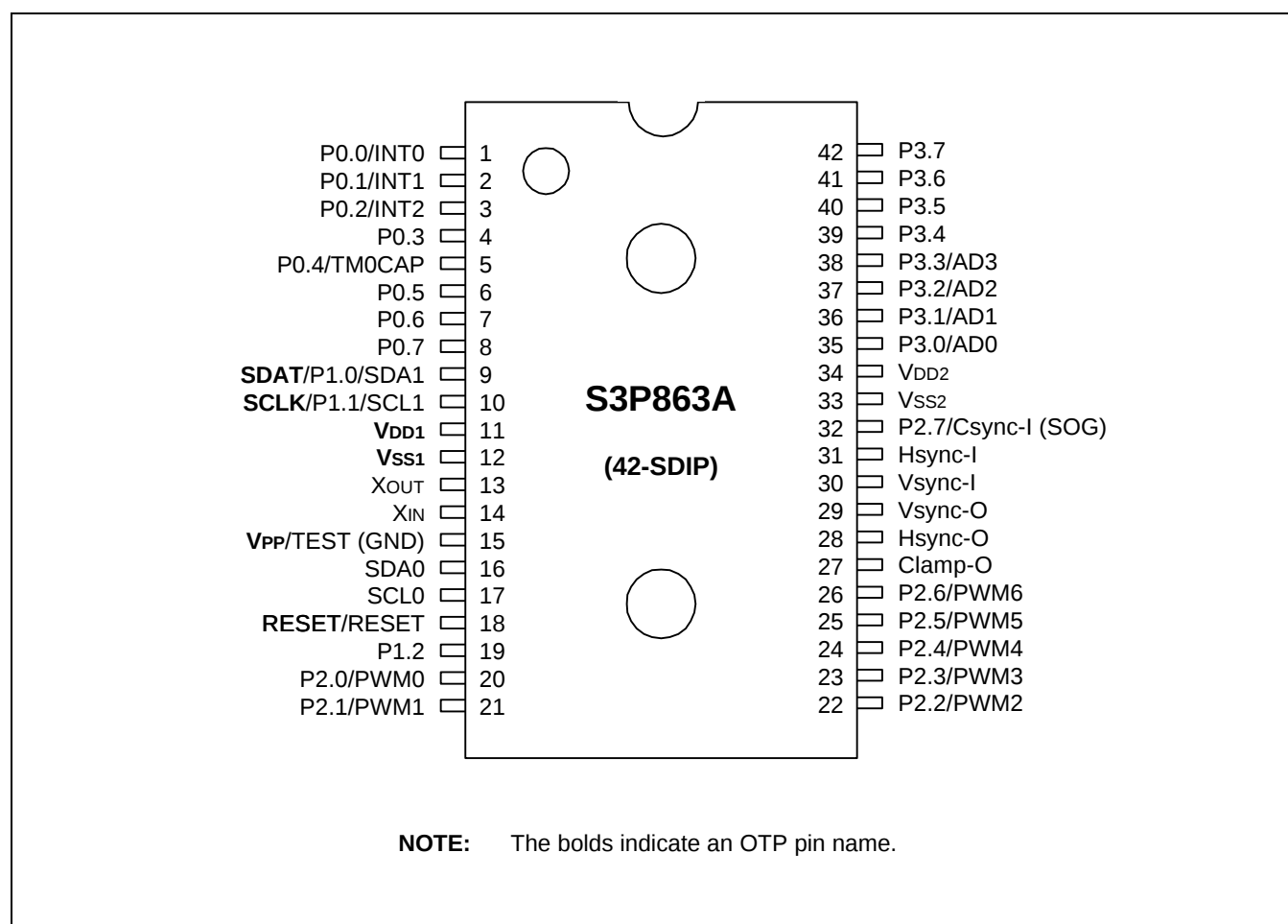
Figure 21-1. S3P863A Pin Assignments (42-SDIP Package)
