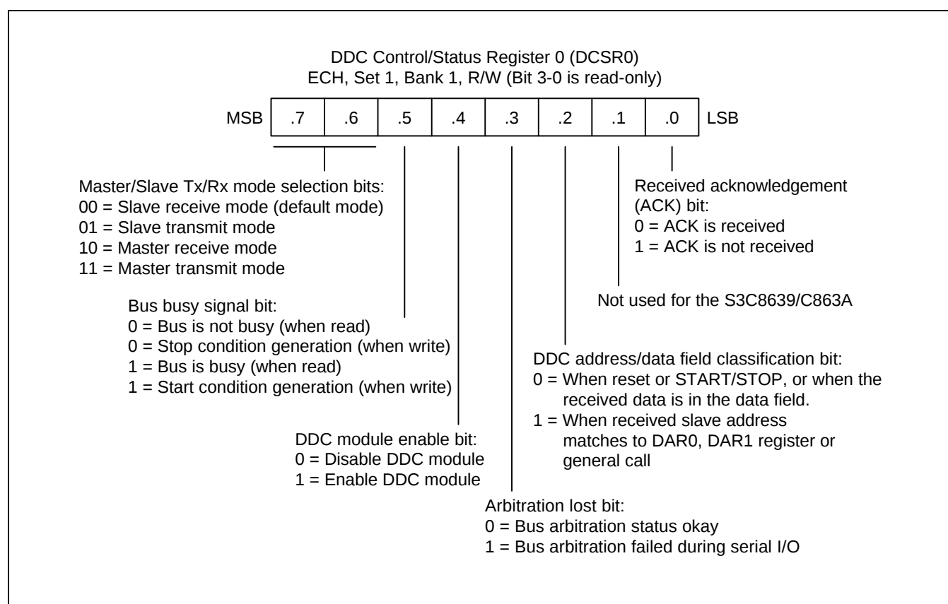
Figure 17-3. DDC Control/Status Register 0 (DCSR0)
