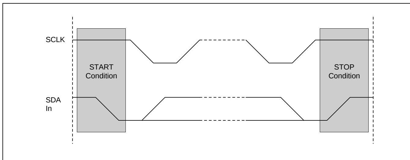
Figure 17-12. Start and Stop Conditions
