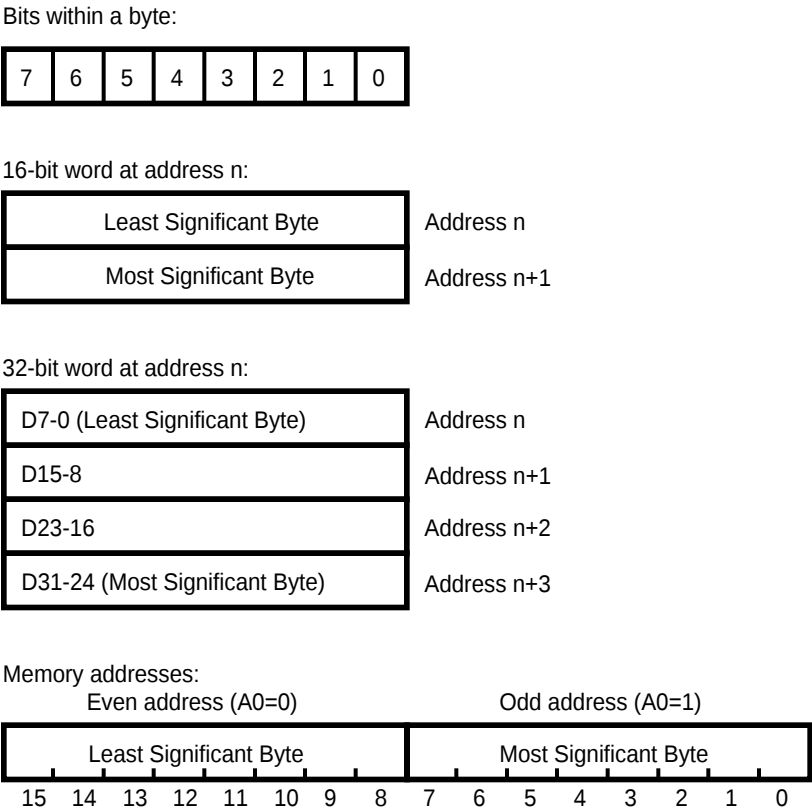
Figure 23. Bit/Byte Ordering Conventions
