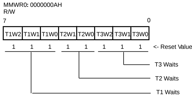
Figure 42. Mid-range Memory Waits Register 0
