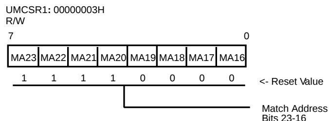
Figure 35. Upper Memory Chip Select Register 1
