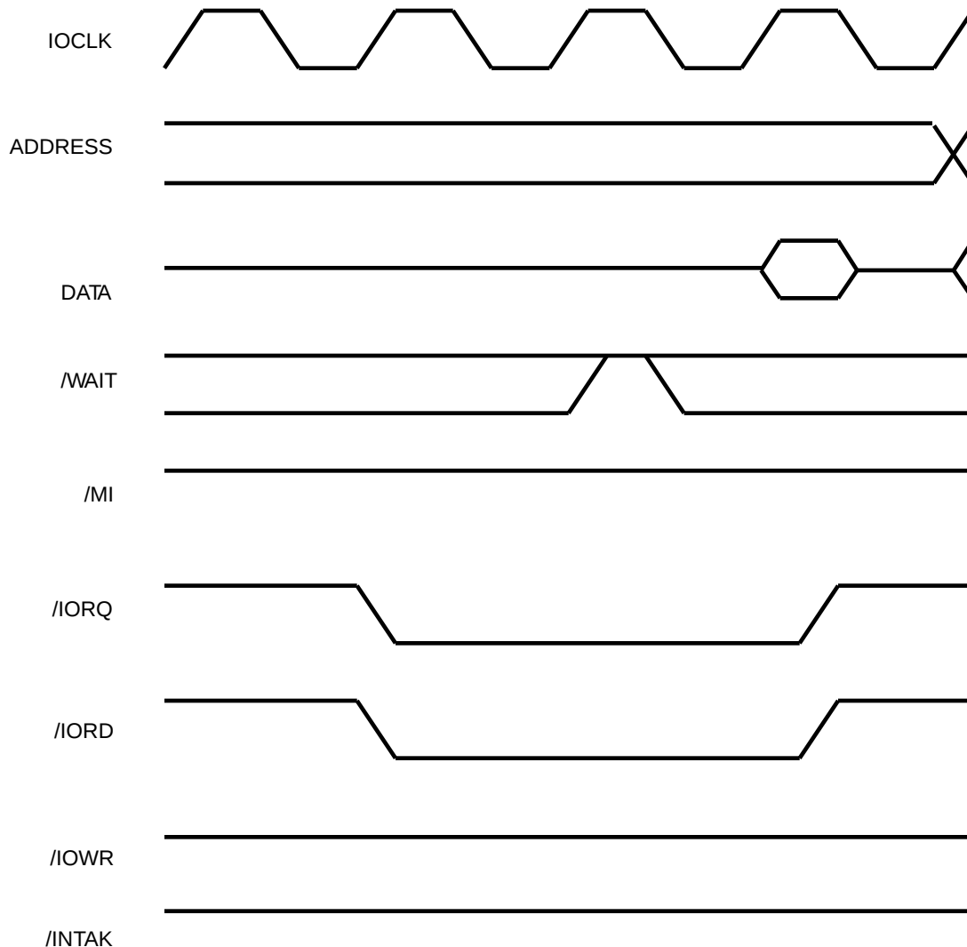
Figure 8A. I/O Read Cycle, No Waits
