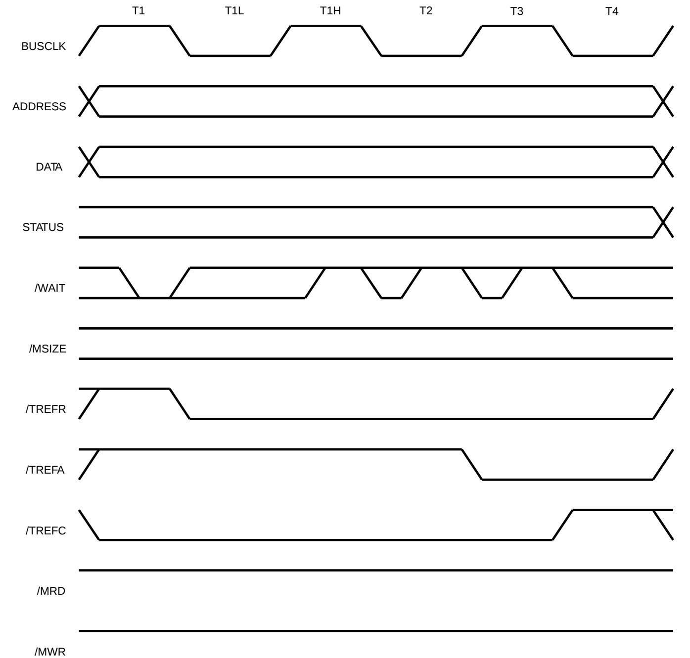
Figure 6B. Refresh Cycle, T1 Wait
