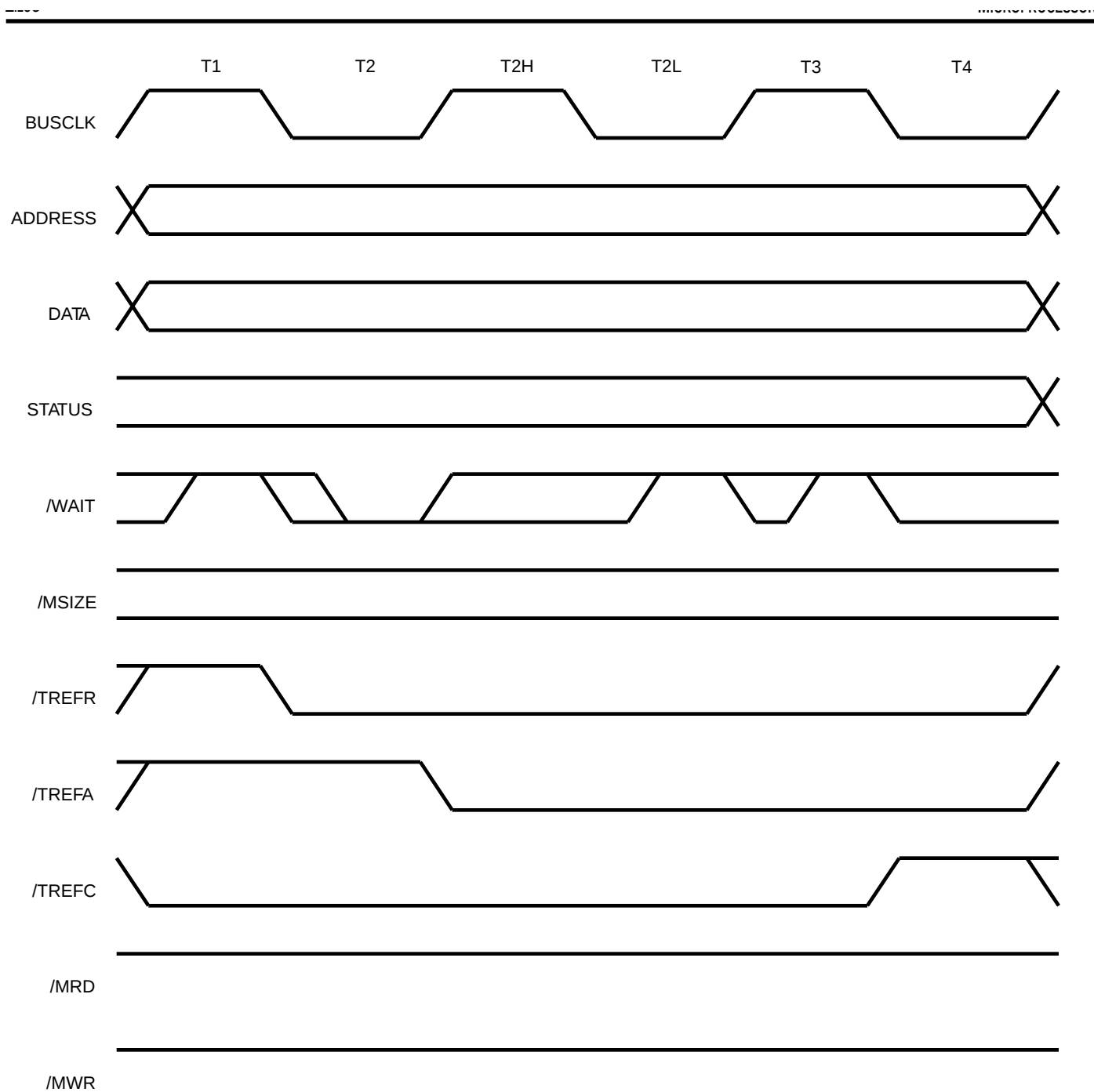
Figure 6C. Refresh Cycle, T2 Wait
