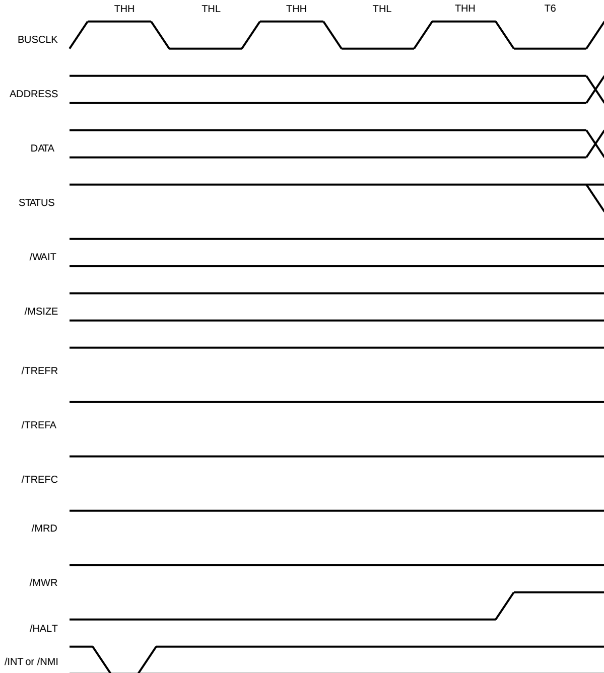
Figure 13. HALT Exit
