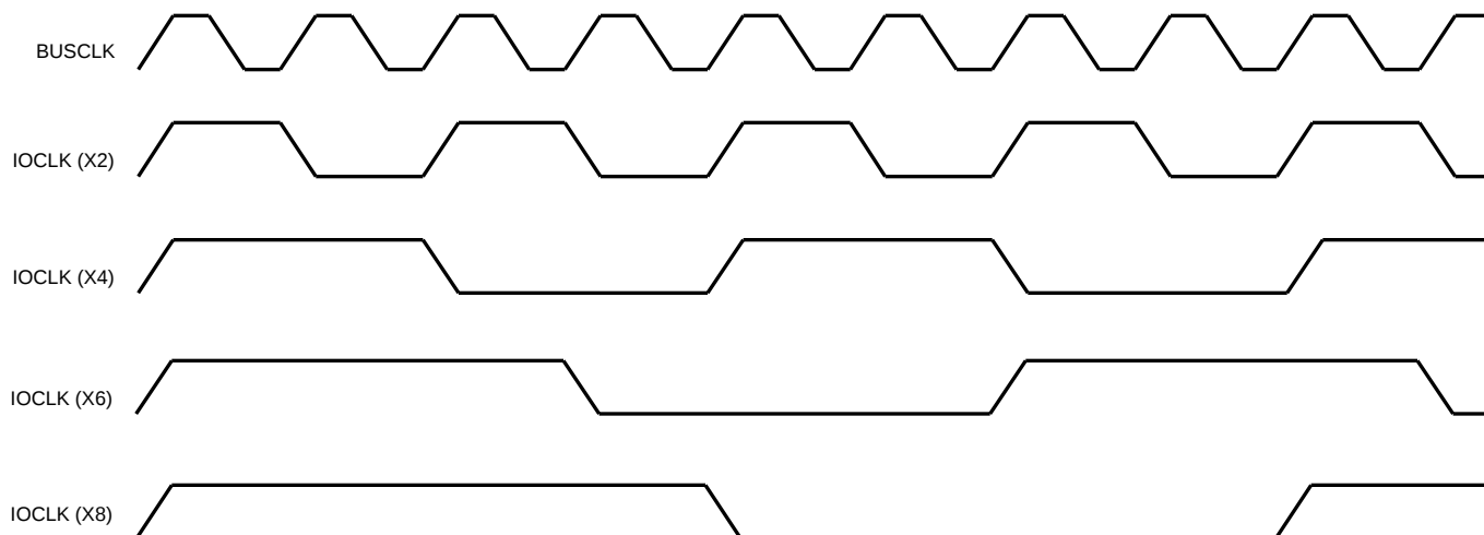
Figure 7. IOCLK Timing
