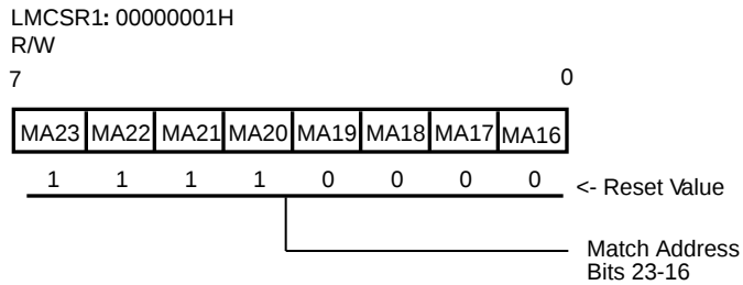
Figure 33. Lower Memory Chip Select Register 1
