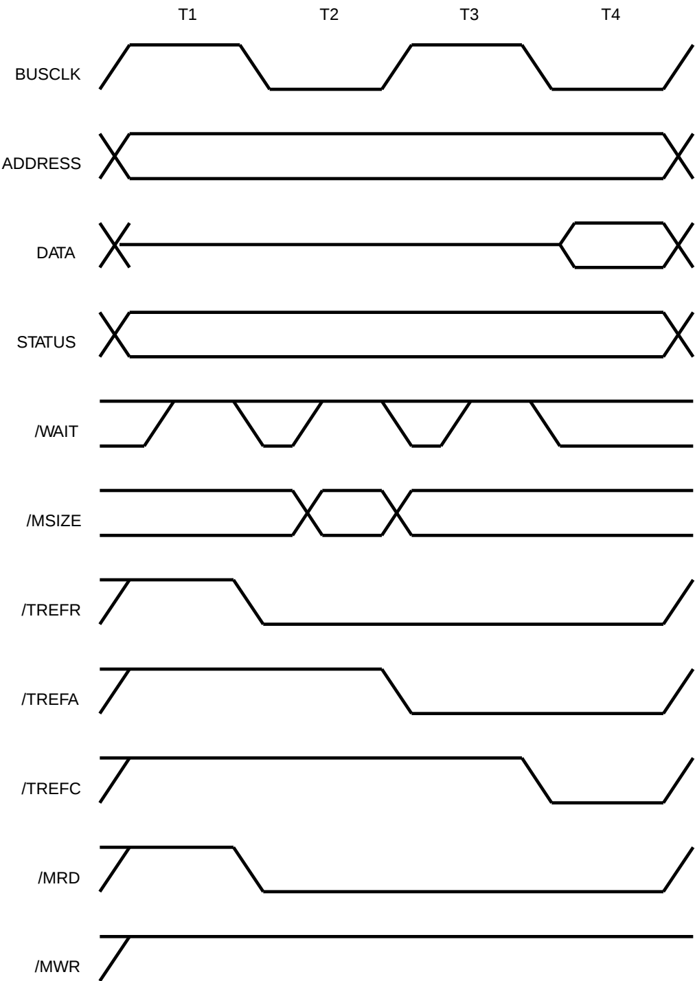
Figure 3A. Read Cycle, No Waits
