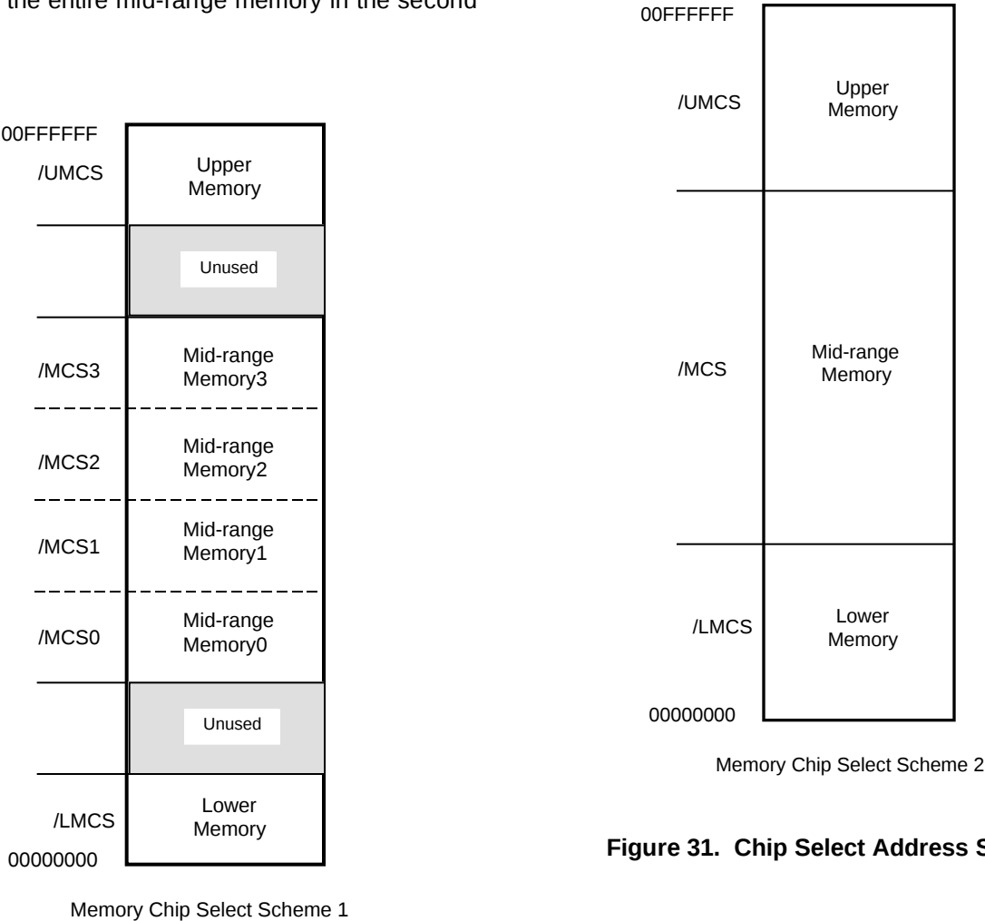
Figure 30. Chip Select Address Space
