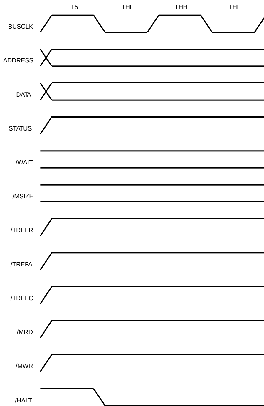
Figure 12. HALT Entry
