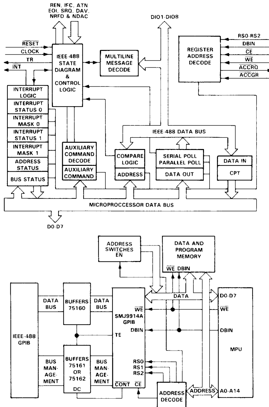
FIGURE 1. TYPICAL SMJ9914A APPLICATION
