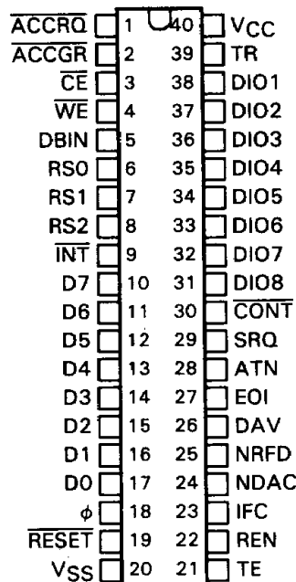
JD PACKAGE (TOP VIEW)
