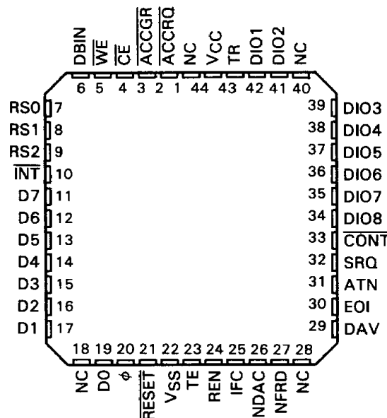
FD PACKAGE (TOP VIEW)
