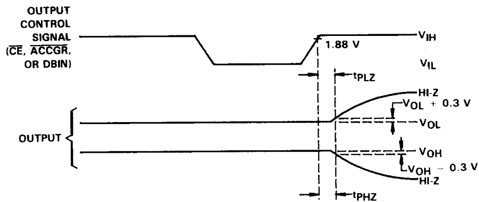
FIGURE 5. HIGH-IMPEDANCE MEASUREMENTS
